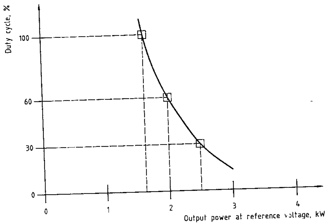
Figure B.1 — Example of duty cycle related to output power at reference voltage
